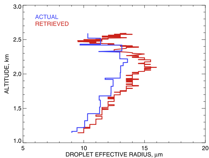
Fig. 3. Vertical profiles of effective radius (left) and variance (right) of droplet size distributions along the illuminated cloud side (red curve in Fig. 2). Blue curves show the actual values from LES model output, while red curves depict retrievals from virtual RSP measurements using the parametric fit method. (For interpretation of the references to colour in this figure legend, the reader is referred to the web version of this article.)
