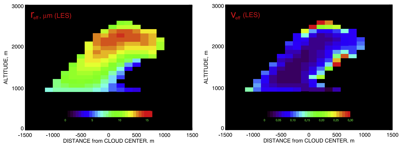
Fig. 4. Actual (from LES model) distribution of effective radius (left) and variance (right) values within the cloud cross-section being studied. The size of the pixels represents the resolution of the LES model.
