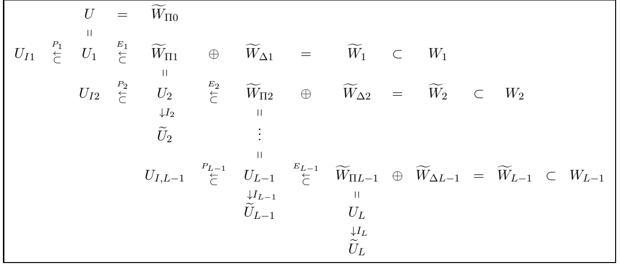
Figure 1: Space decompositions, embeddings and projections in the Multilevel BDDC
