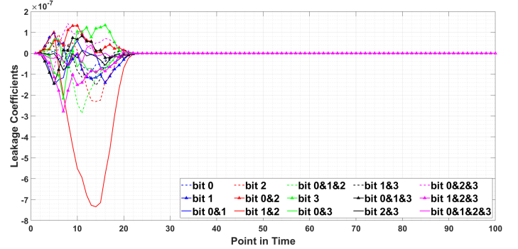
Fig. 4: Leakage coefficients of the ISW extracted with respect to the number of samples per unit of measurement.
