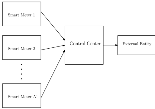
Fig. 1 Network model
