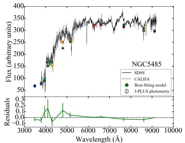
Fig. 11. Comparison between the integrated spectra in a 3" diameter fiber of SDSS, CALIFA, and the photo-spectrum of J-PLUS for NGC 5485. Error bars correspond to the photometric errors. The best-fitting model to the photo-spectrum of J-PLUS is plotted as green circles. The bottom panel shows the residuals of the best-fitting model.
