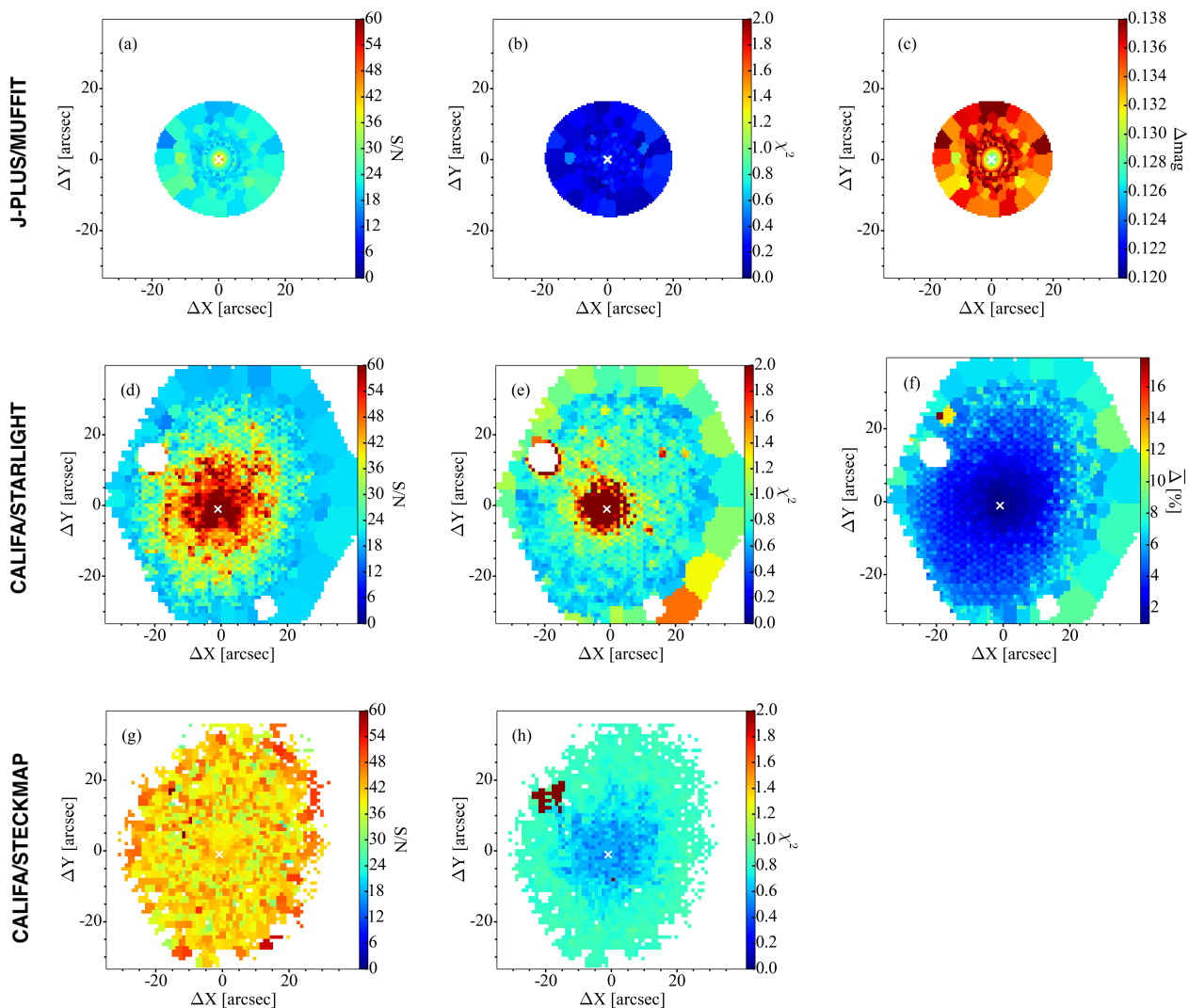
Fig. 5. Maps with data and fit quality indicators for NGC 5473 determined by J-PLUS/MUFFIT (top panels), CALIFA/STARLIGHT (middle panels), and CALIFA/STECKMAP (bottom panels). The center of the galaxy is indicated with a white cross in each panel.
