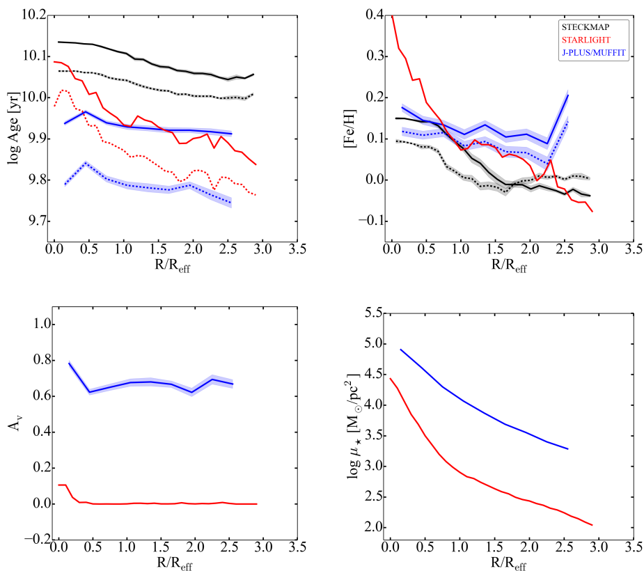
Fig. 8. Mass-weighted (solid lines) and luminosity-weighted (dashed lines) radial profiles for NGC 5473 of log Age, [Fe/H], A_v , and \log \mu_* for the three different methods. Enclosed shadowed regions correspond to the uncertainties of each profile.
