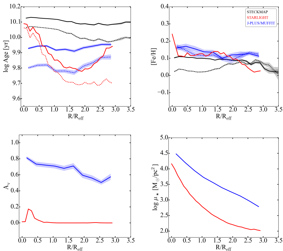
Fig. 9. Same as in Fig. 8, but for NGC 5485.
