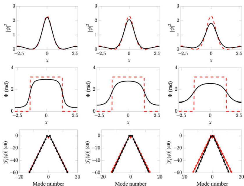
Task 6, Figure 1. Comparison of cnoidal wave solutions with (black-solid) and without (red-dashed) loss for a five-period solution. The solutions with and without loss resemble each other in this case. [Qi et al. J. Opt. Soc. Am. B 34 , 785 (2017).]
