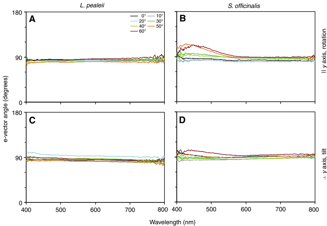
Fig. 4. Spectra of e-vector angles of the arm stripes of the squid and the cuttlefish oriented parallel (A,B) or perpendicular (C,D) to the y-axis. Data collected in Position 2 (see Fig. 1). As in Fig. 3, different colored spectra represent the calculated results from samples at various tilt or rotation angles (key in A also applies to B–D).
