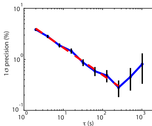
Figure 7. The normalized Allan–Werle deviation as a function of averaging time ( \tau ) demonstrates the precision benefit of time averaging up to 250 s. Fitting the data with \tau < 250 s yields a slope of -0.5 (dashed red line), which is consistent with white noise dominating the variability at shorter averaging periods. [\text{HCHO}] = 5 ppbv.
