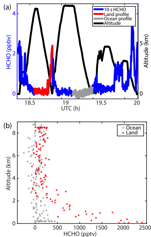
Figure 12. Flight data for AJAX flight 185 on 19 April 2006. (a) Time series of HCHO (10 s data, blue) and the corresponding aircraft altitude (black), with spiral profiles over land (red) and ocean (gray) highlighted. (b) Altitude profiles of HCHO (10 s data) over land (red) and ocean (gray).
