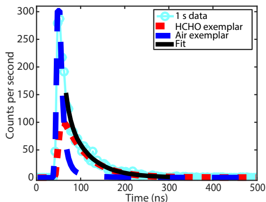
Figure 5. Each 1 s data profile (cyan circles) is fit using a linear combination of the air (dashed blue line) and HCHO (dashed red line). The fit profile, over the time window used for the least squares fit, is shown in black. The HCHO mixing ratio is 8 ppbv.
