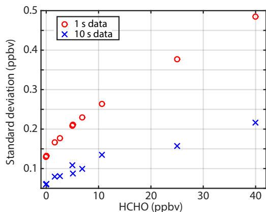
Figure 6. The standard deviation as a function of HCHO is shown to demonstrate the precision of the HCHO measurement for 1 and 10 s averaging.
