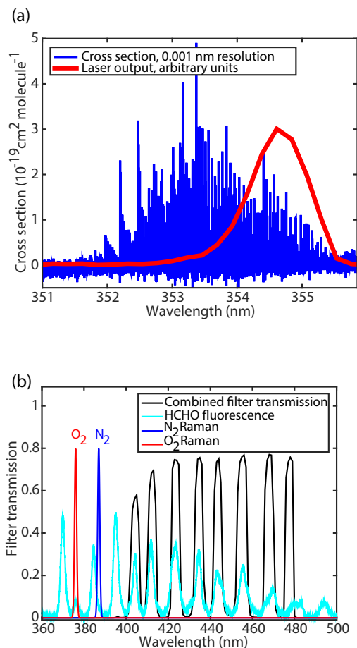
Figure 1. (a) The HCHO absorption spectrum (Co et al., 2005), averaged to 0.001 nm resolution, and the excitation laser spectrum are shown. (b) The optical filter transmission spectrum is shown for the detection axis 2 (multi-band-pass filter). The HCHO fluorescence and the \text{N}_2 and \text{O}_2 Raman spectra are included for reference, all with arbitrary units.
