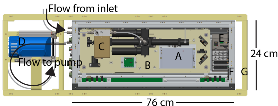
Figure 2. COFFEE instrument layout in the AJAX pod rack, including the (a) laser, (b) optical plate, (c) pressure controller, (d) vacuum pump, (e) RIO data acquisition system, (f) instrument chassis, and (g) AJAX pod rack.
