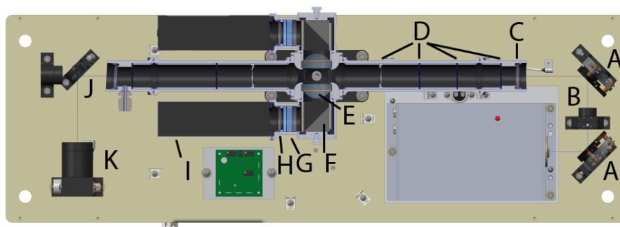
Figure 3. The optical plate layout is shown, with a cutaway of the detection cell. The components include the (a) steering mirrors, (b) half-wave plate and collimating lens, (c) cell windows, (d) laser baffles, (e) aspheric lens, (f) prism dielectric mirror, (g) optical filters, (h) lens, (i) photomultiplier tube, (j) beam splitter, and (k) laser power monitor.
