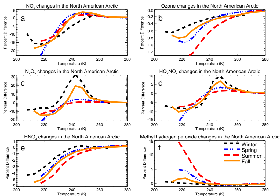
Fig. 4. Differences between the GEOS-Chem base case and MPN case ( ((\text{MPN}-\text{BASE})/\text{BASE}) \times 100 ) over the North American Arctic versus temperature for (a) NO x , (b) ozone, (c) N 2 O 5 , (d) HO 2 NO 2 , (e) HNO 3 , and (f) methyl hydrogen peroxide. These results are temperature binned means of 24 h averaged concentrations.
