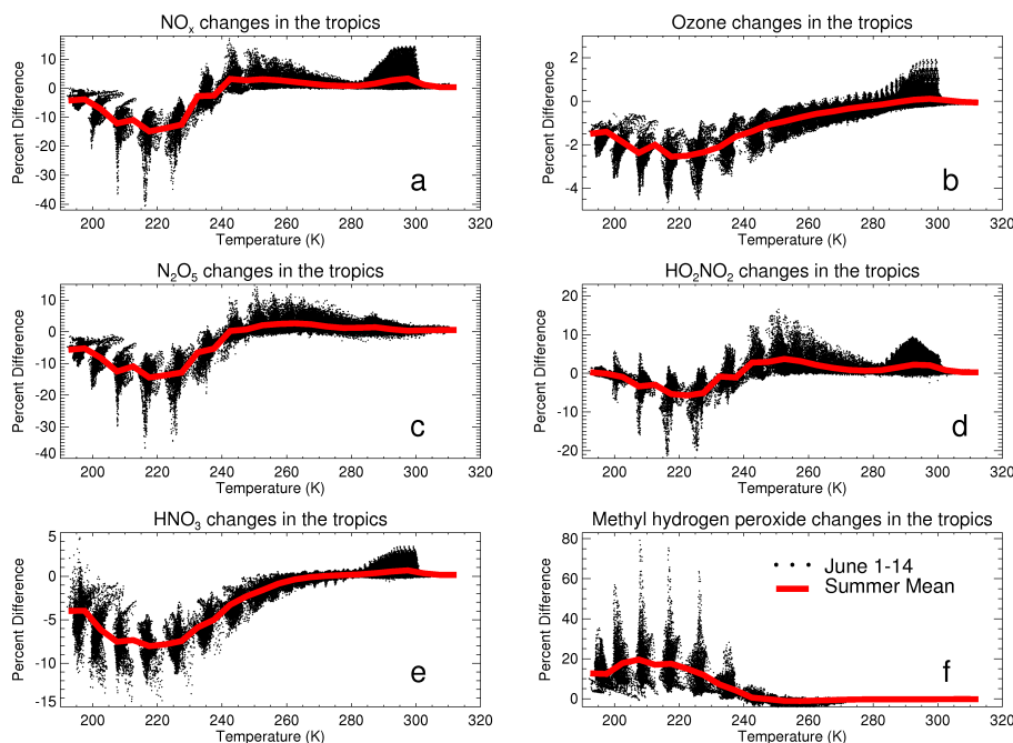
Fig. 6. Differences between the GEOS-Chem base case and MPN case ( ((\text{MPN}-\text{BASE})/\text{BASE}) \times 100 ) over the tropics versus temperature for (a) \text{NO}_x , (b) ozone, (c) \text{N}_2\text{O}_5 , (d) \text{HO}_2\text{NO}_2 , (e) \text{HNO}_3 , and (f) methyl hydrogen peroxide. The individual points are the 24 h average value of 1–14 June 2008. The red line is the summer mean concentration. The regular temperature intervals at low temperatures are a result of decreasing vertical resolution in the model at increasing altitudes.
