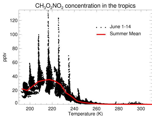
Fig. 5. Tropospheric concentrations of CH 3 O 2 NO 2 versus temperature over the tropics. The individual points are the 24 h average value of 1–14 June 2008. The red line is the summer mean concentration. The regular temperature intervals at low temperatures are a result of decreasing vertical resolution in the model at increasing altitudes.
