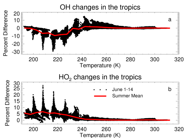
Fig. 7. Differences between the GEOS-Chem base case and MPN case ( ((\text{MPN}-\text{BASE})/\text{BASE}) \times 100 ) over the tropics versus temperature for (a) OH and (b) \text{HO}_2 . The individual points are the 24 h average value of 1–14 June 2008. The red line is the summer mean concentration. The regular temperature intervals at low temperatures are a result of decreasing vertical resolution in the model at increasing altitudes.
