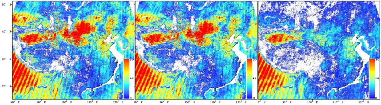
Figure S1. Annual frequency of MISR (left) small, (middle) large-mode AOD, and MISR AOD >0.15 (right), respectively.
