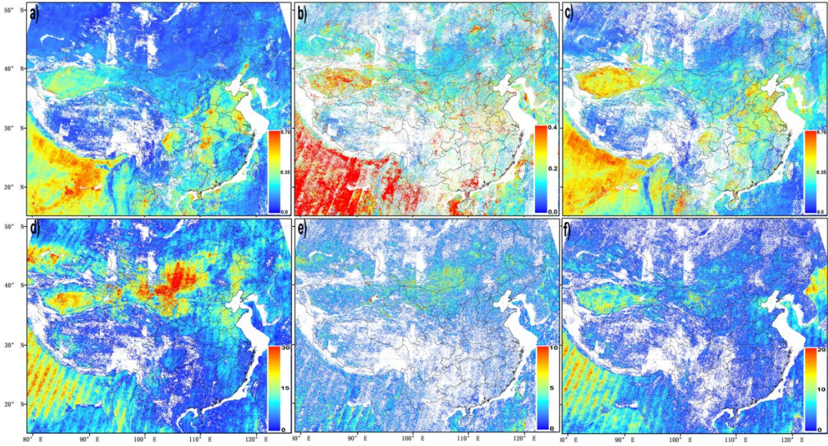
Figure S3. Annual mean of MISR AOD in mixture group a) 1-30, b) 31-50, and c) 51-74, and d-f) their frequency, respectively.
