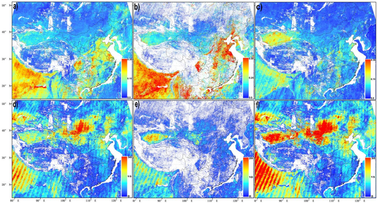
Figure S2. Annual mean of MISR spherical nonabsorbing AOD with effective radius a) \leq 0.12 \mu\text{m} , b) at 0.26 \mu\text{m} , and c) 2.8 \mu\text{m} , and d-f) their respective frequency.
