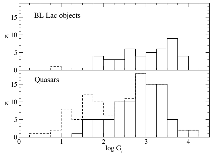
Figure 4. Distribution of \gamma -ray to radio luminosity ratio for BL Lac objects (top panel) and quasars (bottom panel). Upper limit values for AGNs with no Fermi ILAC catalog associations are indicated by the dashed lines.
