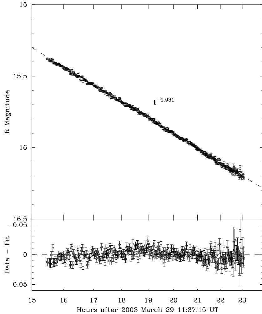
FIGURE 1. Top: R-band light curve of the GRB 030329 afterglow. Bottom: Difference between data and model.
