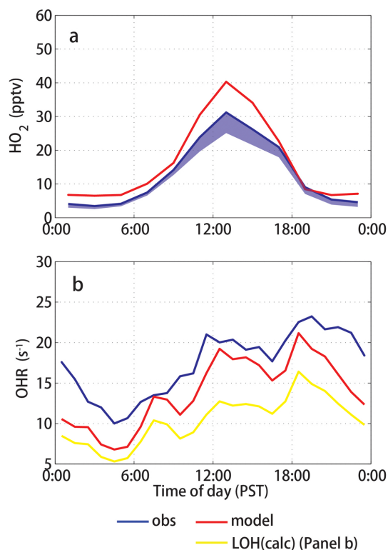
Fig. 4. Diurnal cycle of \text{HO}_2 (a) and OH reactivity (b) between 20 June and 30 July 2009 near the Blodgett Forest Research Station (BFRS). In the top panel, the shaded area below measured \text{HO}_2 (blue solid line) indicates the contribution to measured \text{HO}_2 from an \text{RO}_2 interference from isoprene, MVK and MACR (Fuchs et al., 2011). In the bottom panel, the calculated OH reactivity from available measurements (LOH) is represented by a yellow line. The absolute uncertainty of the \text{HO}_2 measurements is \pm 40\% at 2\sigma confidence. The absolute uncertainty of OH reactivity measurement is 1 \text{ s}^{-1} at 2\sigma confidence (Mao et al., 2009). The model incorporates the current understanding of BVOC oxidation chemistry (see text for details).
