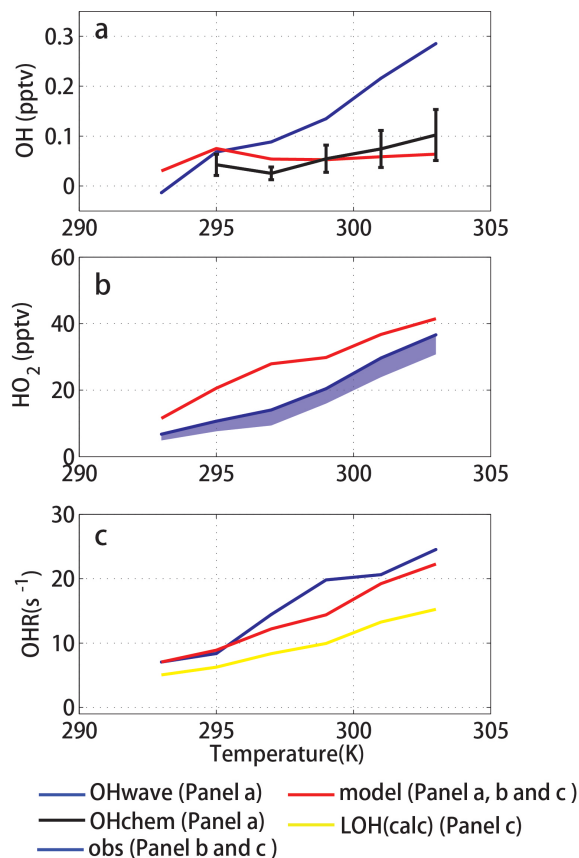
Fig. 5. Temperature dependence of (a) daytime measured and modeled OH, (b) daytime measured and modeled \text{HO}_2 , and (c) OH reactivity between 9:00 and 15:00 PST during BEARPEX09. In (a), OHwave (blue line), OHchem (black line) and modeled OH (red line) agree at low temperature, but OHwave has a significant temperature increase while OHchem and modeled OH show little temperature dependence. The vertical bars indicate a combined uncertainty as described in Fig. 2. Note that OHchem here is corrected by 0.80 to account for the removal of internal OH by \text{C}_3\text{F}_6 addition (see supplemental material). In (b), measured \text{HO}_2 (blue line) is lower than modeled \text{HO}_2 (red line) but not significantly at the low and high temperatures. Measured \text{HO}_2 may be affected by an \text{RO}_2 interference from isoprene, MVK and MACR (Fuchs et al., 2011), as indicated by the blue shading. In (c), the difference between the measured OH reactivity (blue line) and the OH reactivity calculated from available measurements (yellow line) suggests missing OH reactivity, which is mostly resolved when including modeled intermediates (red line) in the calculation.
