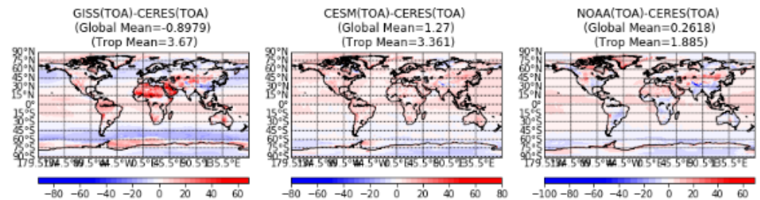
Fig: Shortwave Radiation Bias for Clear Sky
