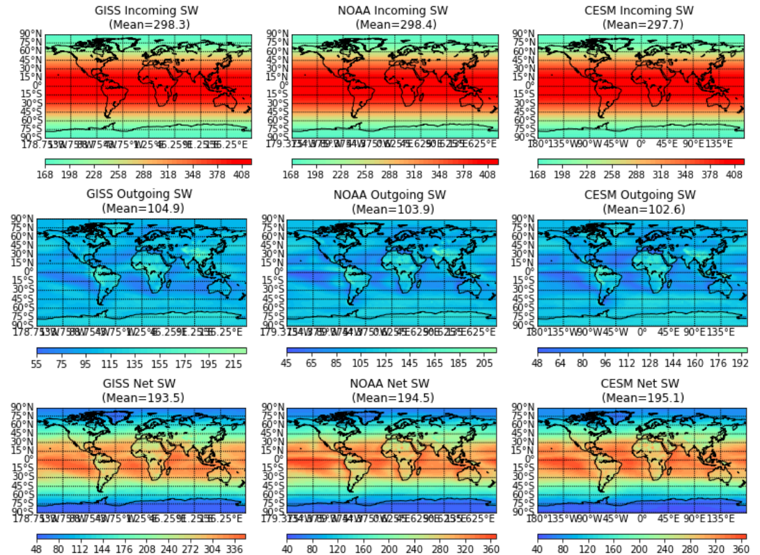
Fig: Shortwave radiation flux for All Sky
