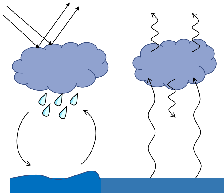
Cloud feedbacks
