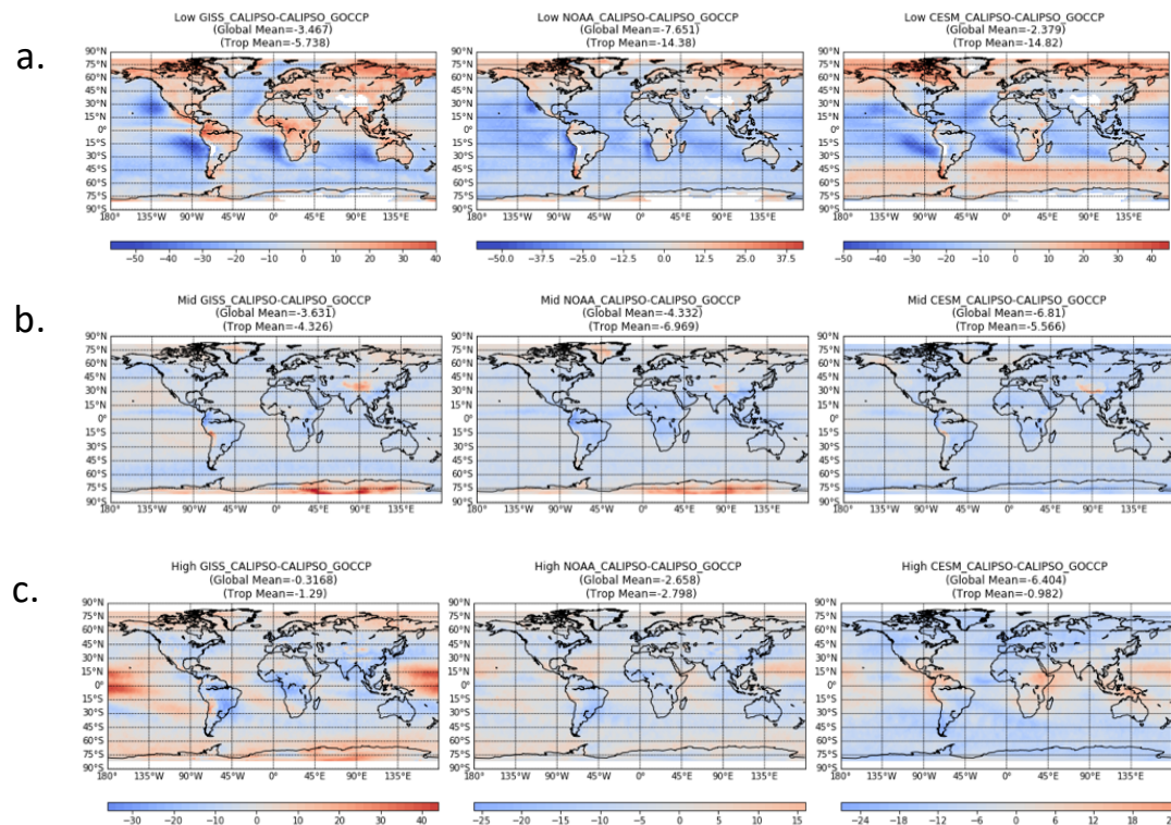
Fig: a. Low, b. Mid, and c. High Cloud Fraction Bias
