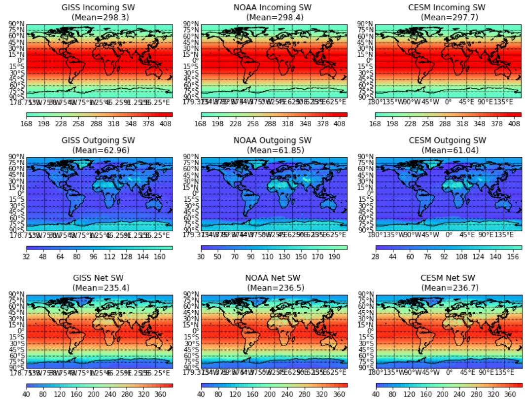
Fig: Shortwave radiation flux for Clear Sky
