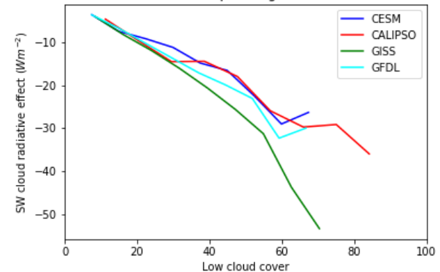
Shortwave cloud radiative effect variation with low cloud cover Tropical region
