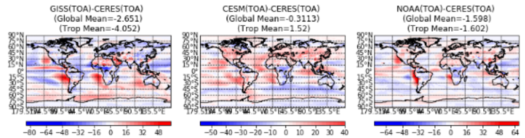
Fig: Shortwave Radiation Bias for All Sky
