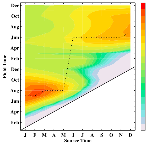
Figure 2. Seasonal evolution of the BIRs at 80°N and 420 K as a function of source time and field time. The dotted line indicates the time of the peaks of the BIRs.
