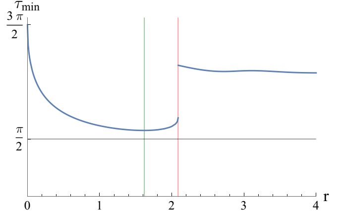
FIG. 3. Minimal time \tau_{\min} to complete a qubit flip in \mathcal{Q} as a function of r = \Omega/\omega . The first vertical line (green) marks the optimal ratio r_{\text{opt}} \approx 1.620000 that leads to the fastest computation \tau_{\min}^{(\text{opt})} \approx 1.807022 . The second vertical line (red) denotes a critical point r_{\text{crit}} \approx 2.087532 , where \tau_{\min} discontinuously increases. Further, for r \rightarrow \infty we see that \tau_{\min} asymptotically approaches \tau_{\min}^{(r \rightarrow \infty)} \approx 3.332162 . The horizontal line is a reference line that represents the ideal case of a minimal \tau_{\min} for N = 1 .
