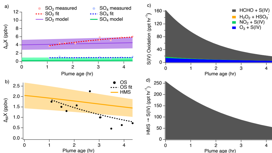
Figure 8. First pass measurements shown by the markers and measurement fits shown by the dashed lines compared to the model results represented by the solid lines with shading denoting an estimated 30% model uncertainty for SO 2 and sulfate (a) and OS (b). Stacked modeled S(IV)
