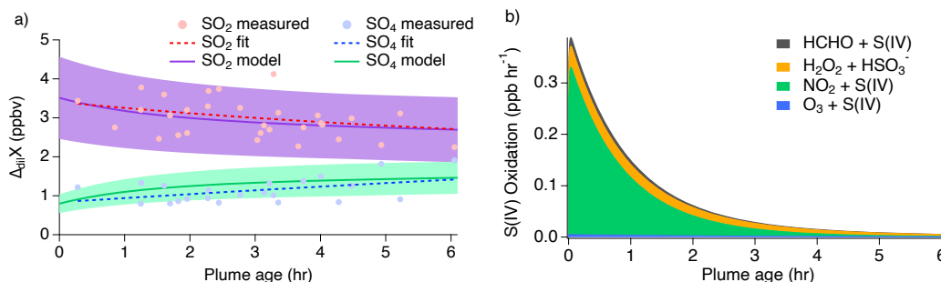
Figure 7. (a) Measurements of 3 August 2019 shown by the markers and measurement fits shown by the dashed lines compared to the \text{SO}_2 and sulfate model results represented by the solid lines with shading denoting an estimated 30% model uncertainty. The sulfate ( \text{SO}_4 ) measurements
