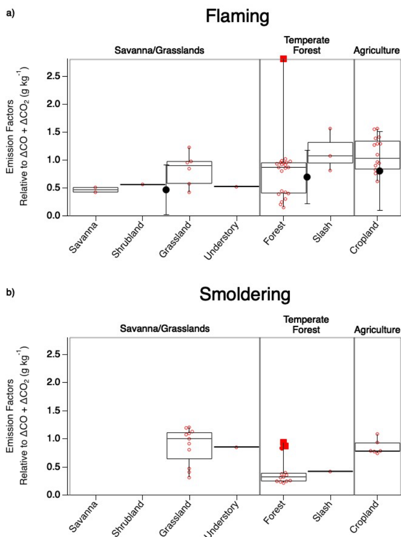
Figure 4. Comparison of \text{SO}_2 EF values observed during flaming (a) and smoldering (b) combustion across fuel types sampled during FIREX-AQ. The box upper edge represents the 75 th percentile and the lower edge the 25 th percentile with the median shown by the middle line. The whiskers represent the minimum and maximum observed values with the open circles representing each observation and the solid red circle representing a potential outlier. The large solid black circles with error bars depicting 1 standard deviation in panel (a) show corresponding average Andreae (2019) values.
