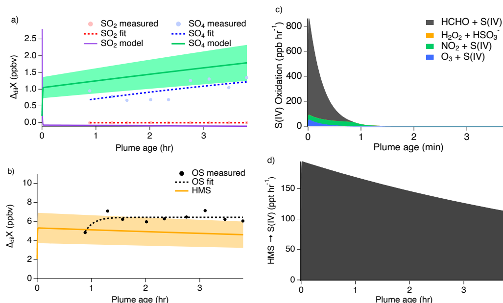
Figure 9. Second pass measurements shown by the markers and measurement fits shown by the dashed lines compared to the model results represented by the solid lines with shading denoting an estimated 30% model uncertainty for \text{SO}_2 and sulfate (a) and OS (b). Stacked modeled S(IV) oxidation rates (c) leading to sulfate and HMS production. HMS reverse reaction rate (d) reproducing S(IV).
