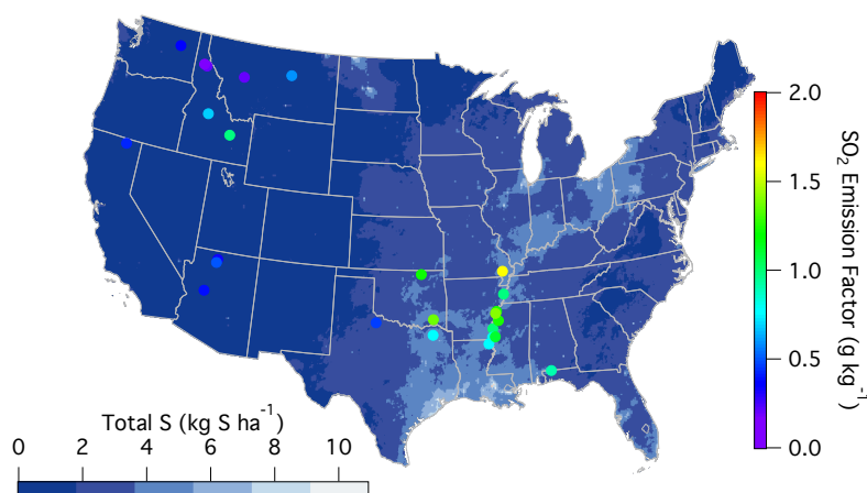
Figure 5. National Atmospheric Deposition Program (2022) reported sulfur deposition rates ( https://nadp.slh.wisc.edu/committees/tdep/#tdep-maps ) compared to SO 2 EFs (closed circles) by geographical location as measured during FIREX-AQ for all fuel types.
