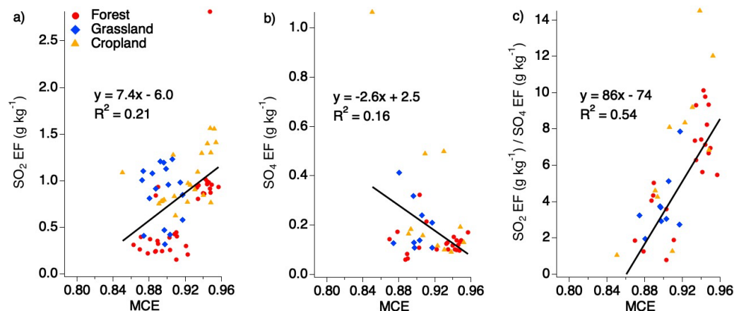
Figure 3. Scatter plots of EFs for \text{SO}_2 (a), sulfate (b), and the ratio of \text{SO}_2 to sulfate (c) (within 1 hr downwind of each fire source) vs. MCE based on combined fuel types.
