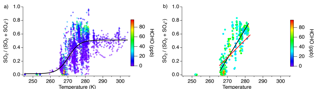
Figure 6. Fractional sulfur conversion as a function of temperature a) including all smoke ages with a sigmoid fit and b) only measurements with \text{HCHO} > 25 \text{ ppb} with the black line indicating the linear fit through the data at all ages between 265–283 K and the red line indicating the linear fit through the measurements within 1 hr of emission in the same temperature regime.
