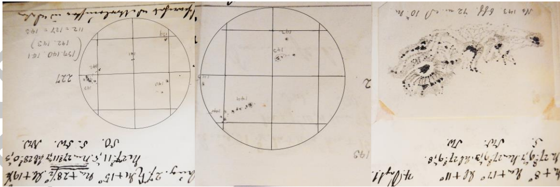
Figure 3: Sunspot drawings by Heinrich Schwabe on August 27 (left), September 1 (centre), and close-up figure of September 1 (right), reproduced from RAS MS Schwabe 31 (p. 131 and p. 136; courtesy of RAS). Circles in the lower halves correspond to the solar disk, on which the sunspots are drawn with the numbers. The sunspot group that caused the Carrington flare is numbered 143 (on left side of the disk in the left panel, and a little upper right of the disk center in the middle panel). Note that Schwabe separated Carrington's Group 520 to Groups 143 and 142. Close-up drawing in the right panel reveals the details of the Group 143. They are reversed as they were seen on the sky. The solar rotational axis is not shown in these drawings. Their limb and contrast have been enhanced here.
