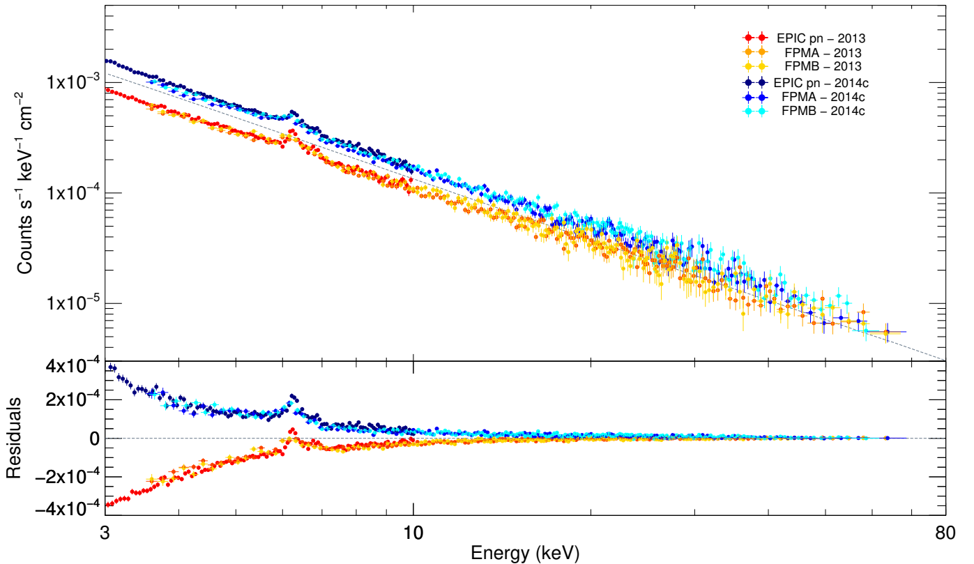
Fig. 1. Simultaneous XMM-Newton and NuSTAR spectra and residuals to a power law model (in counts \text{s}^{-1} \text{keV}^{-1} \text{cm}^{-2} units) are shown, obtained on February 2013 and March 2014 for Ark 120. Dashed gray line indicate a \Gamma = 1.85 power law model, with a 2-10 keV flux of 3 \times 10^{-11} \text{erg cm}^{-2} \text{s}^{-1} .
