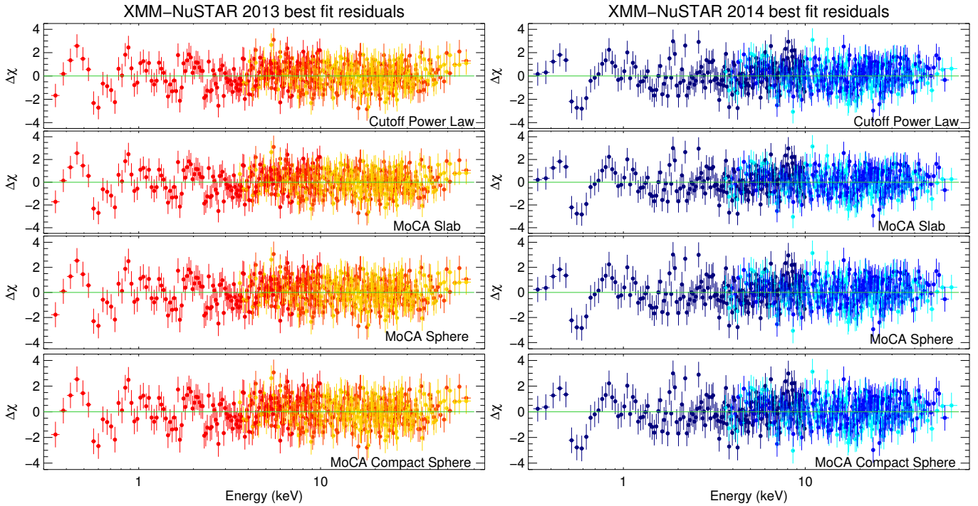
Fig. 2. Residuals for the combined 2013 and 2014 XMM+NuSTAR observations are shown. See text for details about the four models applied. The only residuals present are near to 0.5 keV, which are likely associated to the OI K-shell absorption from our galaxy (see Reeves et al. 2016, for further details).
