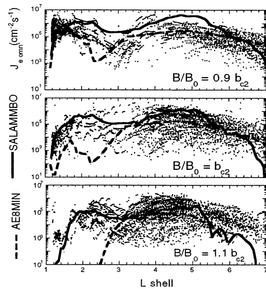
Figure 5. L -shell profiles of trapped electrons (0.19-3.2 MeV) observed by OHZORA at 350-850 km during quiet times ( |ID_{st}| < 30 nT) in 1984-87. The corresponding profiles along three different low altitude trajectories (magnetic cutoffs) as computed from the SalammbO and NASA AE-8MIN models are shown in solid and dashed lines, respectively.
