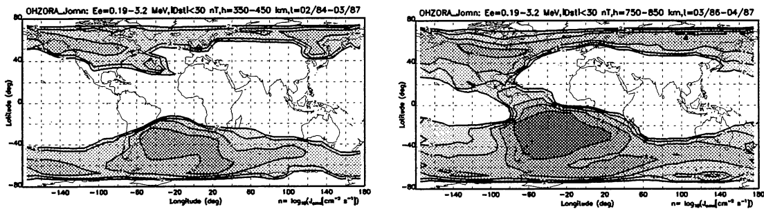
Figure 9. Global distributions of trapped electron (0.19-3.2 MeV) omnidirectional fluxes observed by OHZORA at 400 km (left) and 800 km (right) during quiet times ( |D_{st}| < 30 nT) in 1984-87. The five contour levels vary logarithmically from 10^2 to 10^6 \text{cm}^{-2}\text{s}^{-1} [from Fung et al. , 1996].
