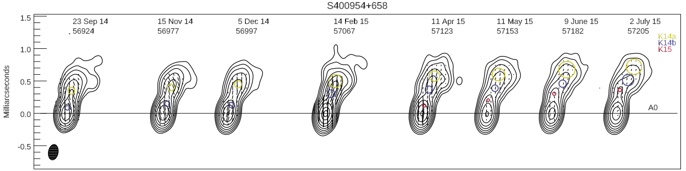
Fig. 4. Sequence of total (contours) and polarized (segments) intensity images of S4 0954+658 at 43 GHz, convolved with a beam of 0.24 \times 0.15 \text{ mas}^2 at \text{PA} = -10^\circ . The global total intensity peak is 1606 \text{ mJy beam}^{-1} and the global polarized intensity peak is 104 \text{ mJy beam}^{-1} ; black line segments within each image show the direction of polarization and their length is proportional to the polarized intensity. The black horizontal line indicates the position of the core, A0, and gray, blue, and red circles show the locations of knots K14a,b and K15, respectively. The size of the circles is proportional to the estimated average size in each epoch. The detailed characteristics of the knots can be found in Table 1 and B.1.
