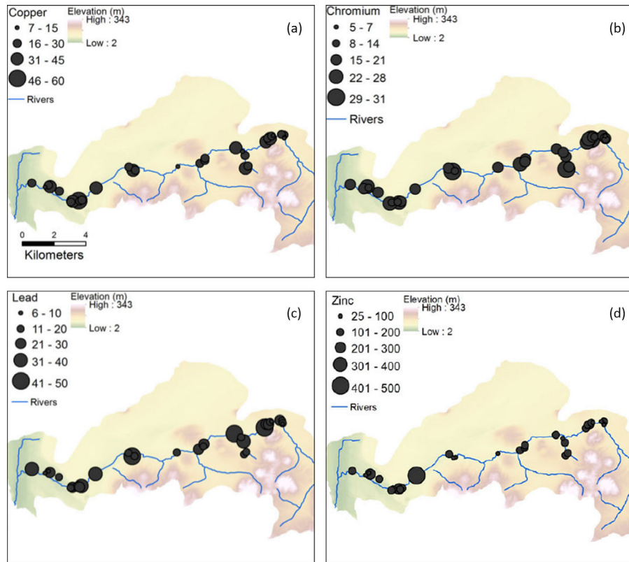
FIGURE 6. Downstream distributions of heavy-metal concentrations (units = ppb) in bed sediments samples around stormwater outfalls in Johnson Creek (a) copper, (b) chromium, (c) lead, and (d) zinc (adapted from Chang et al. 2018). The base maps illustrate the varying topography within the Johnson Creek watershed based on the 10 m Digital Elevation Model (USGS 2015).
