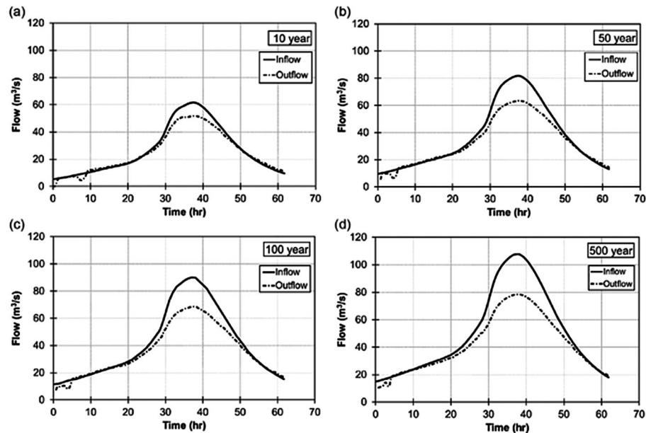
FIGURE 5. Inflow and attenuated outflow hydrographs of the (a) 10-year, (b) 50-year, (c) 100-year, and (d) 500-year flood events in Johnson Creek (from Ahilan et al. 2018).
