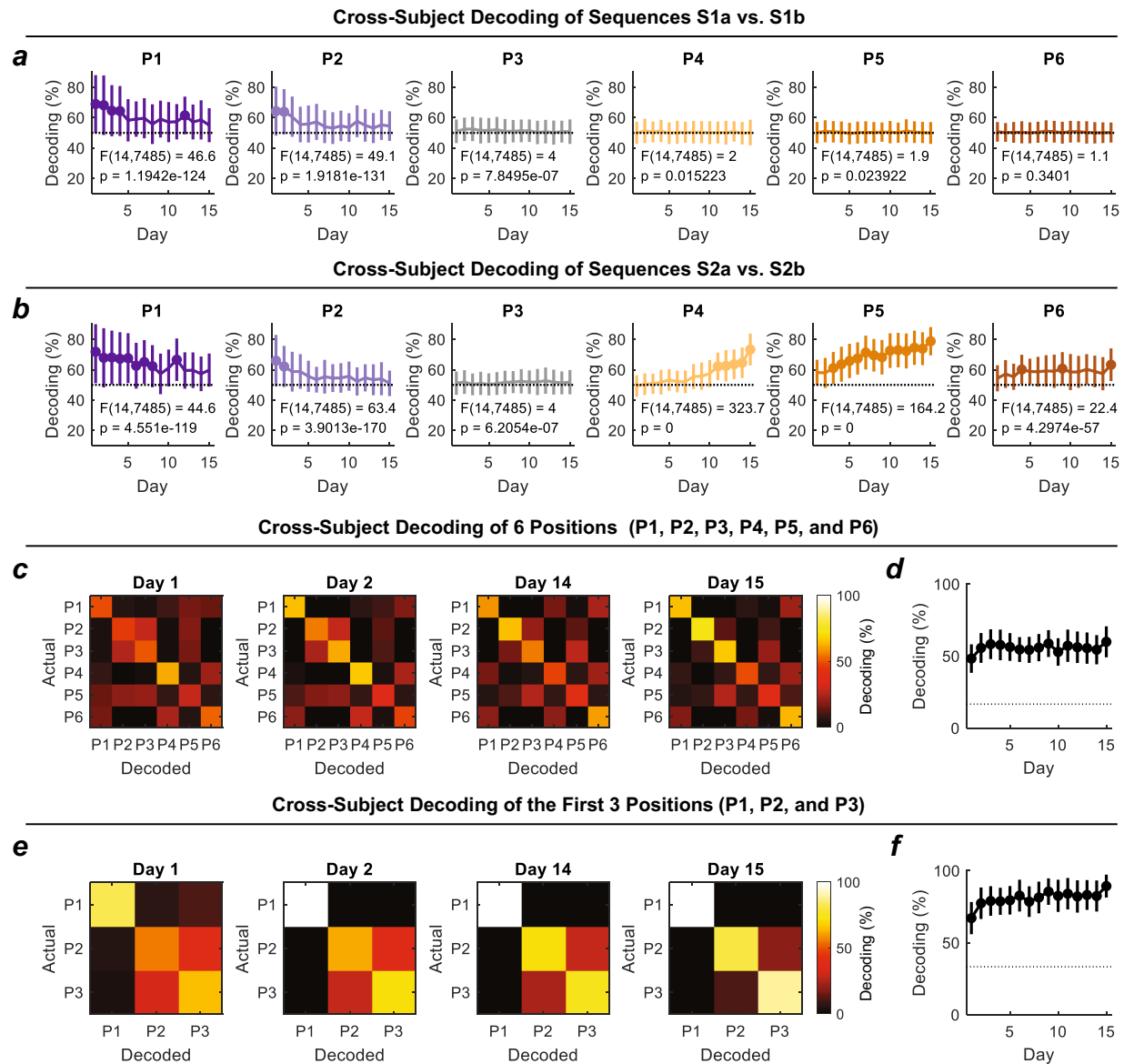
Extended Data Fig. 9 | Cross-subject decoding of sequences and positions.
