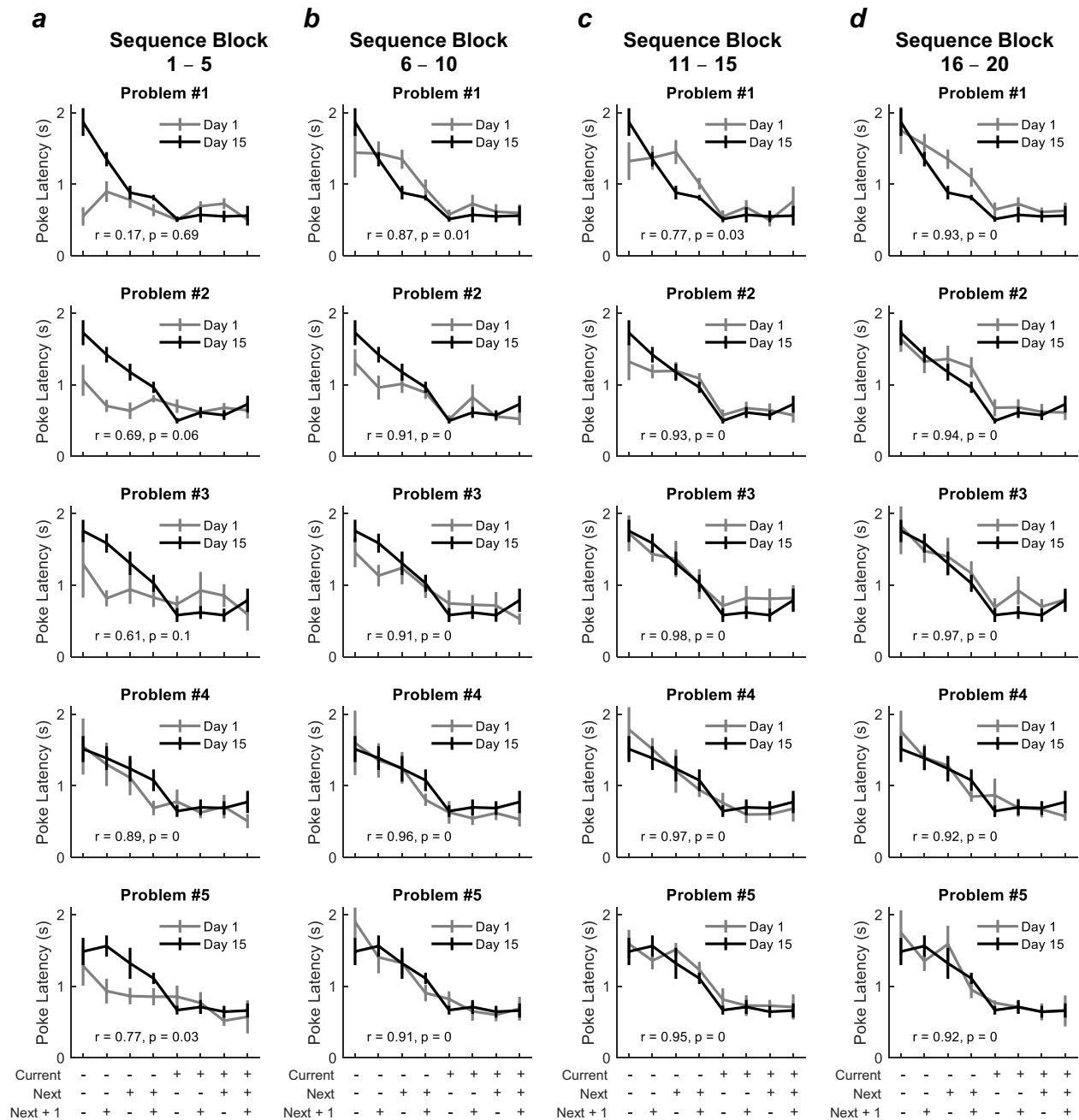
Extended Data Fig. 10 | Comparisons of poke latencies sorted by discounted future reward between day 1 and day 15. a–d , Poke latency measuring the time from the onset of the houselights ('light') to nosepoke ('poke') at the odour port, sorted according to discounted future reward across a : sequence blocks 1–5; b : sequence blocks 6–10; c : sequence blocks 11–15; d : sequence blocks 16–20 on day 1 (grey lines) compared to the poke latencies averaged across all 20 sequence blocks on day 15 (black lines). Each sequence block has 24 trials and comes from 24 trial types. Analyses were performed on
